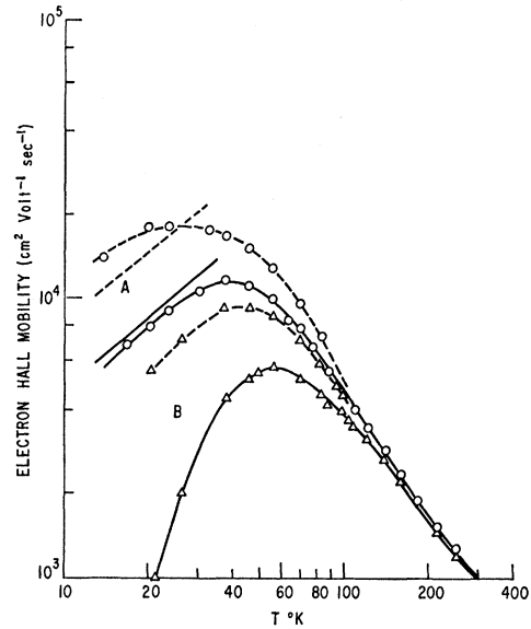
Fig. 2. Electron Hall mobilities for samples shown in Fig. 1. The solid and dashed curves have the same significance as in Fig. 1. The small segments at low temperature are calculated results for the zone-refined sample.
