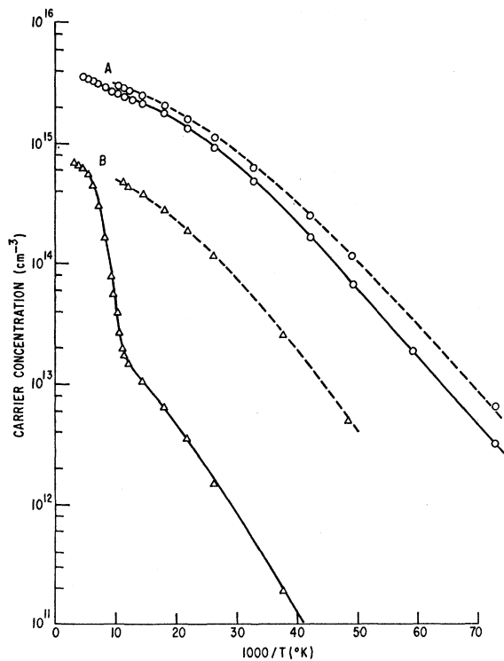
Fig. 1. Typical electron concentrations as a function of temperature. Curves A correspond to a zone-refined sample and B to the same sample quenched after being heated at 900°C in a saturated Cd atmosphere for three minutes. The solid curves represent measurements in the dark and the dashed curves measurements after photoexcitation at low temperatures.
