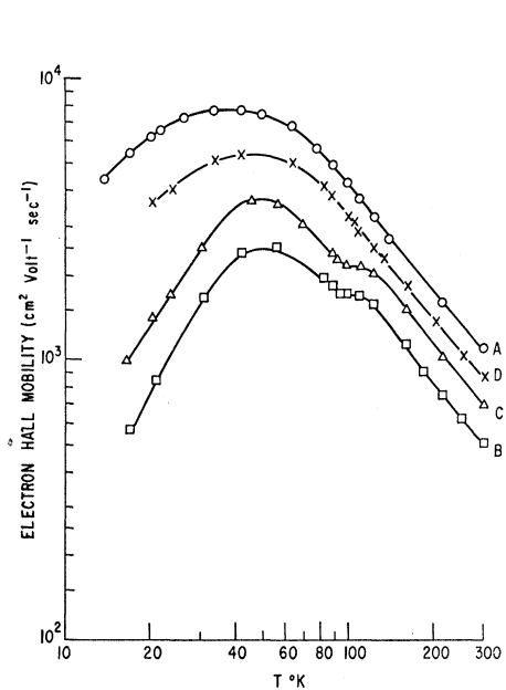
FIG. 5. The Hall mobilities corresponding to samples shown in Fig. 4. The symbols have the same significance as in Fig. 4.
